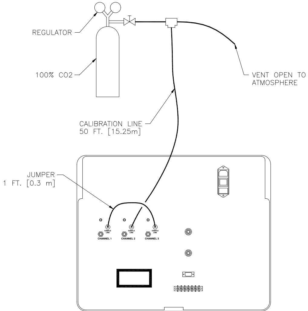
Figure 3 CO 2 Calibration Diagram
