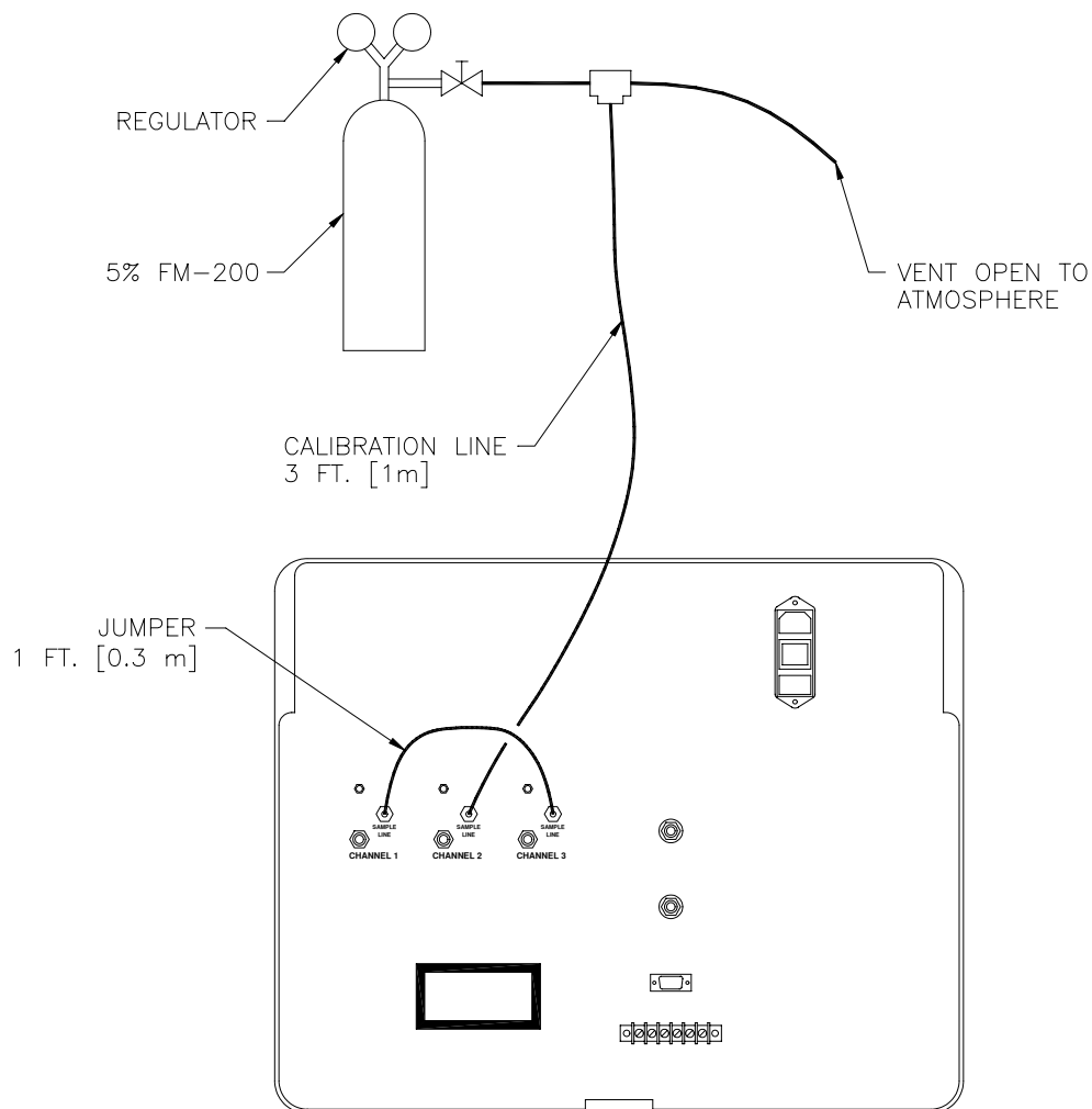
Figure 2 HFC-227ea Calibration Diagram
